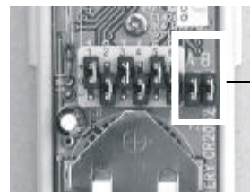
Zone connectors
